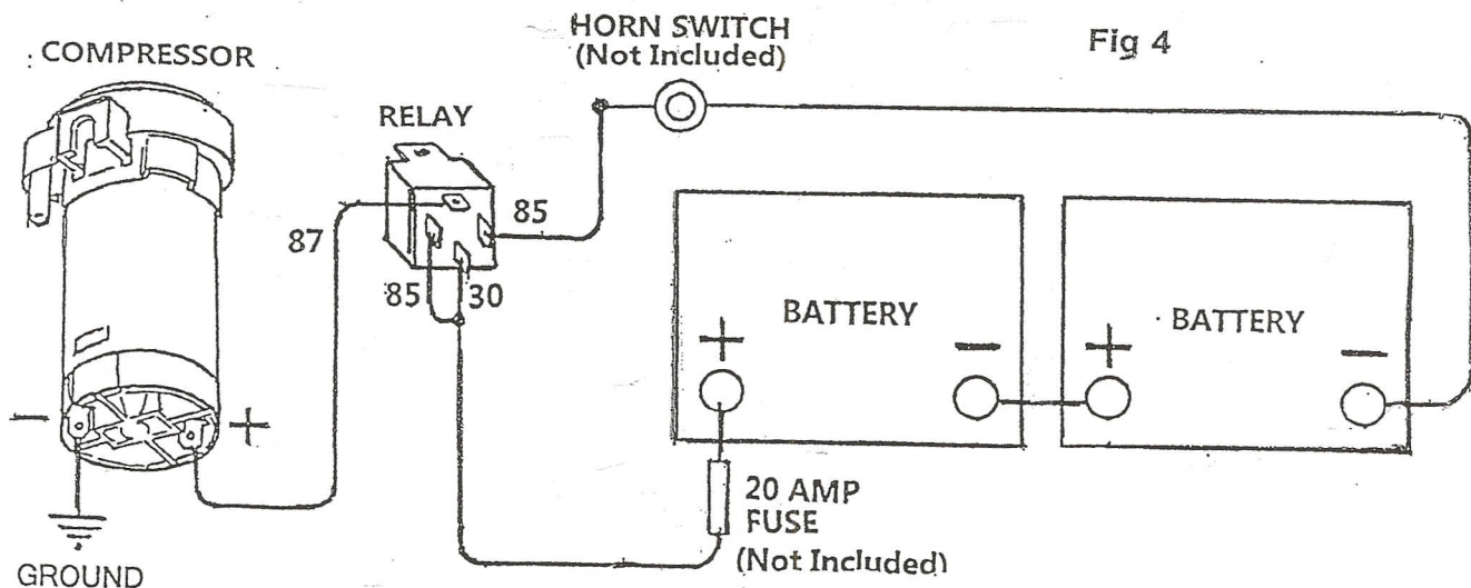
Electrical Connections for a New Horn Button Switch
