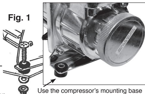
Use the compressor's mounting base as a template to mark the 3/16" holes for drilling
